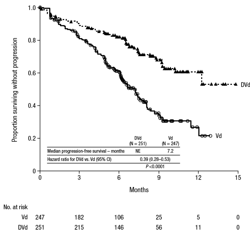
Figure 3: Kaplan-Meier Curve of PFS in Study MMY3004
